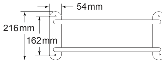
Mounting Specification
